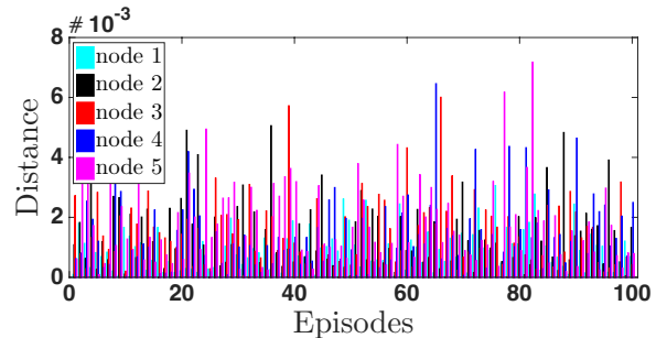
Fig. 5: The Euclidean distance between the local model updates and the global model under the GACE attack.
